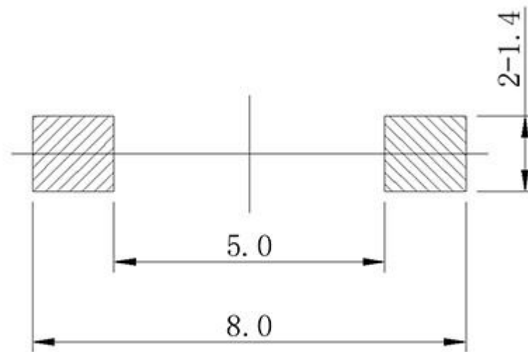
P. C. B LAND DIMENSION
