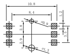
P.C.B电路参考图/Schematic diagram of P.C.B
