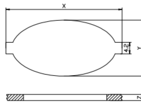
PANEL CUT-OUT
