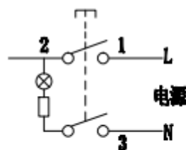
SWITCHING CIRCUIT
